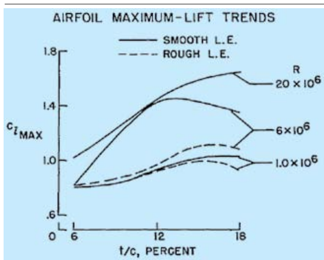
The effect of leading edge smoothness is most pronounced for Reynolds numbers of about 6 million, corresponding to a large boat's rudder at high speed.
